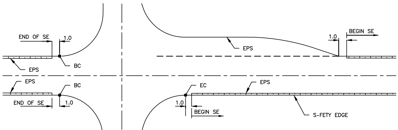
PLAN VIEW - INTERSECTION
