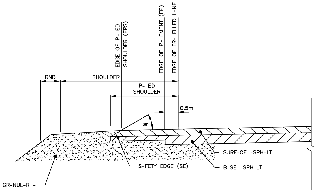
CROSS SECTION
