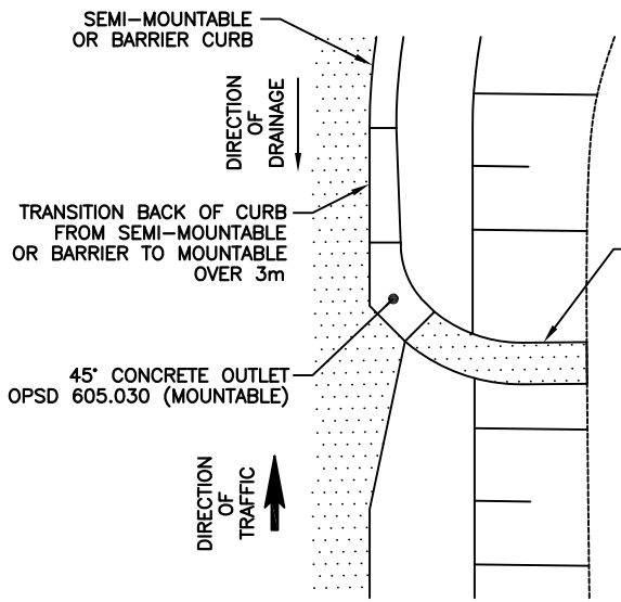
45° CONCRETE OUTLET AT END OF RUN
