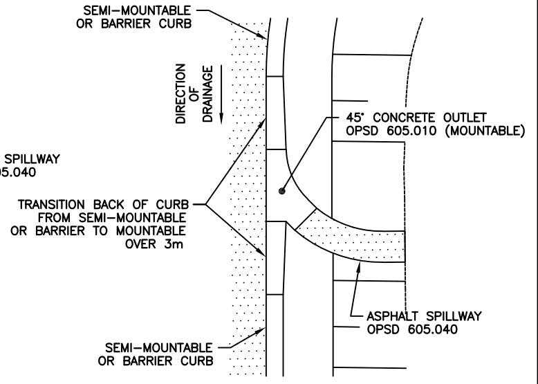
45° CONCRETE OUTLET
