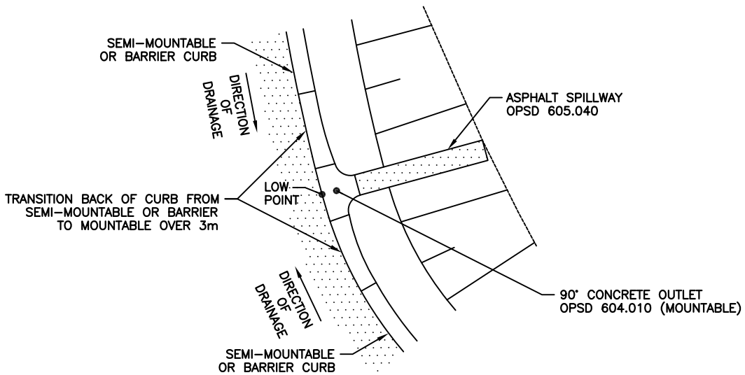
90° CONCRETE OUTLET
