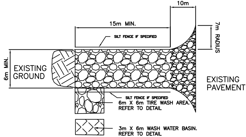
PROFILE VIEW
