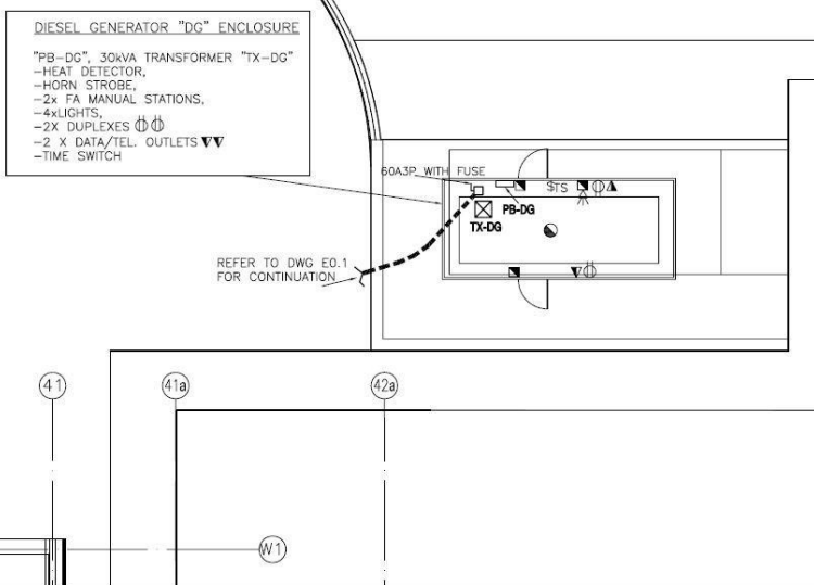
DIESEL GENERATOR PLAN
